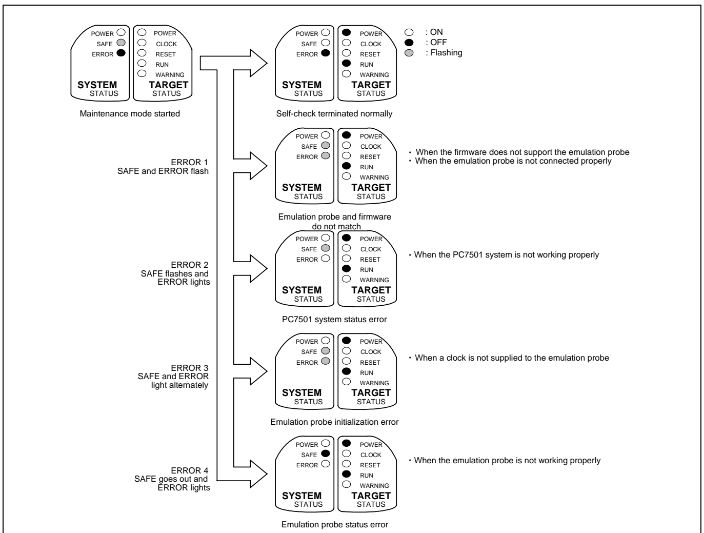
Figure 2.6 Self-check procedure
